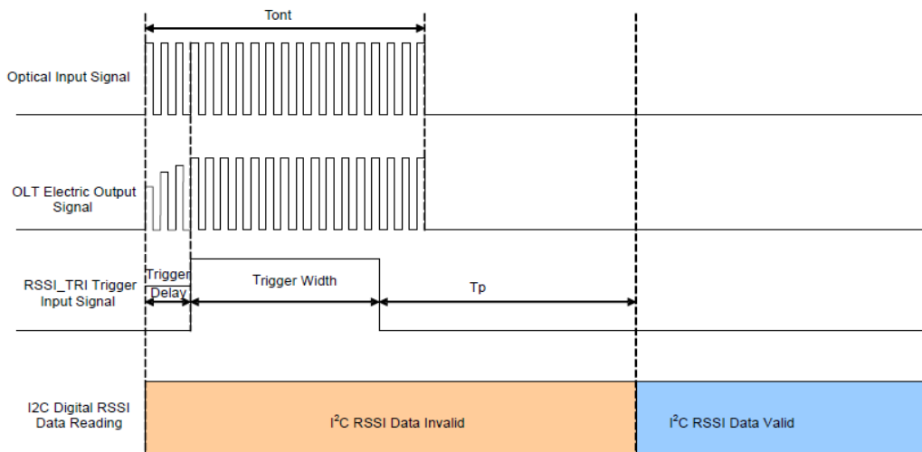
Figure 1 RSSI TIMING SEQUENCE
