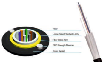
FS-Drop Wire-With Glass Yarn
